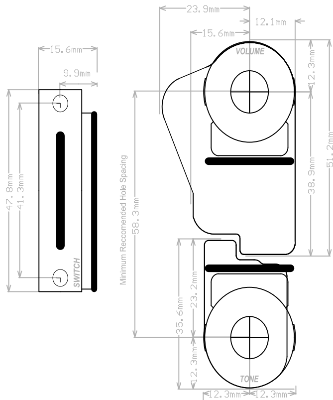
Technical Drawing
